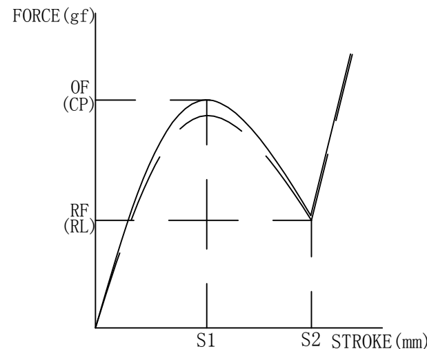
FORCE CHARACTERISTICS
