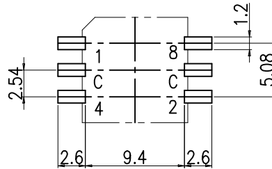
P.C.B DIMENSION (Top View)
