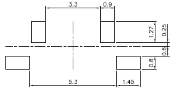
PCB DIMENSION
